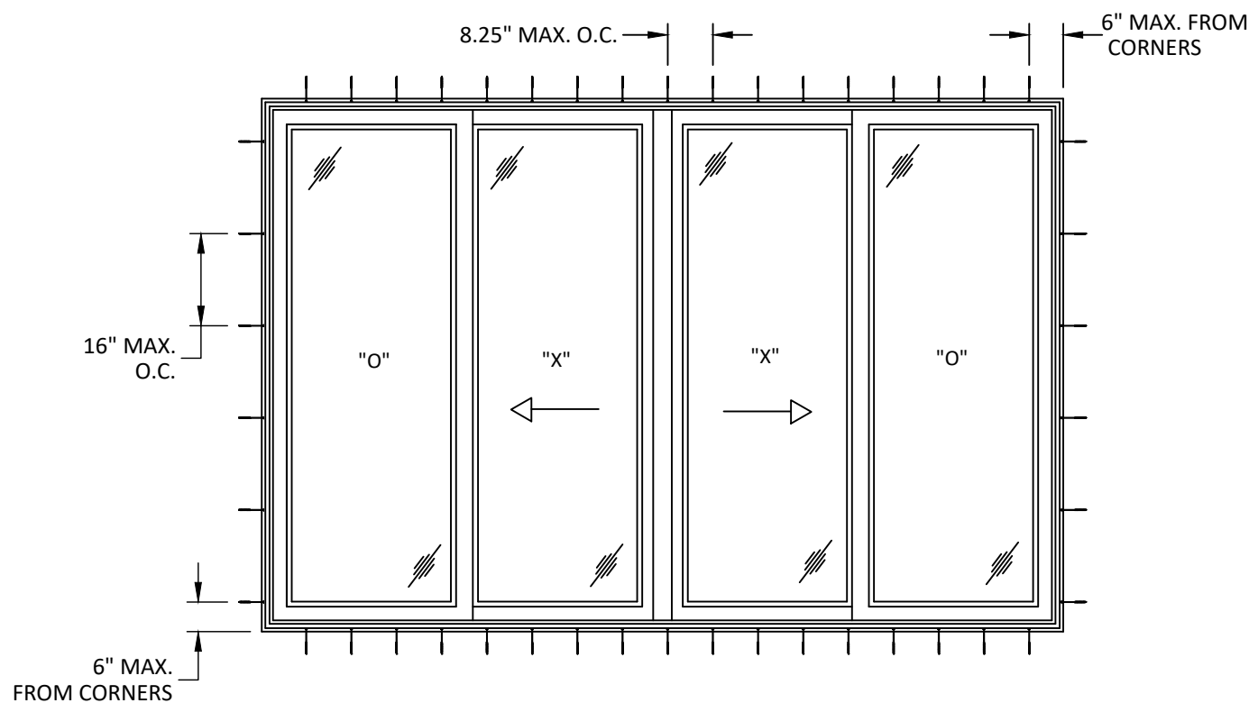
TYPICAL ANCHOR LAYOUT CLIP OR THROUGH FRAME INSTALLATION
