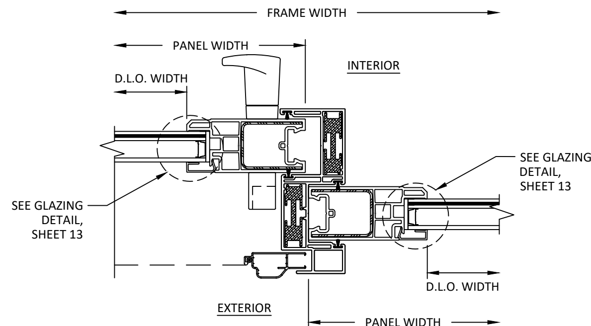
C 12 HORIZONTAL SECTION "OXO" ASTRAGAL
