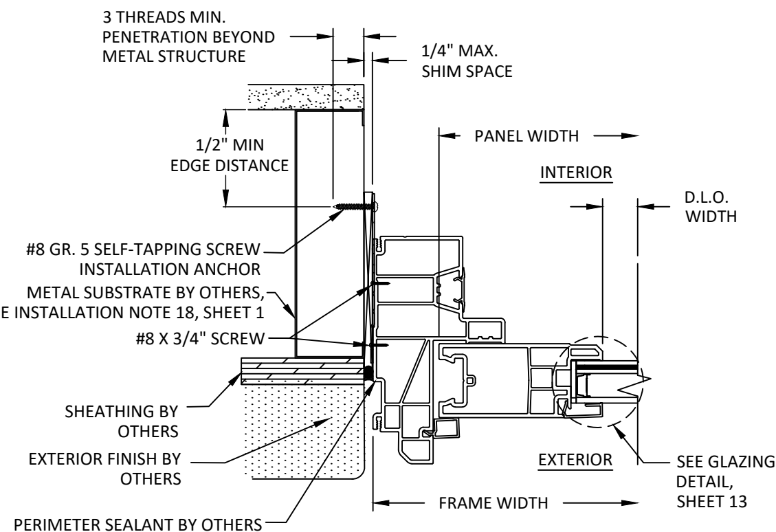
B 11 HORIZONTAL SECTION CLIP INSTALLATION METAL SUBSTRATE
